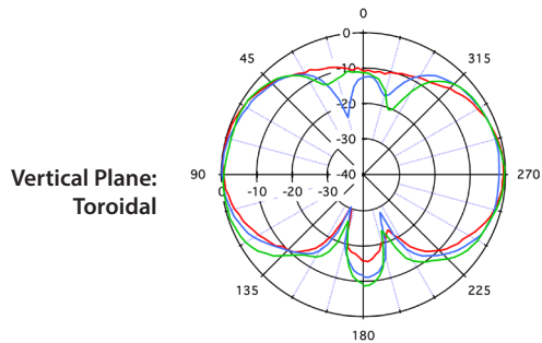
Beamwidth: Vertical
