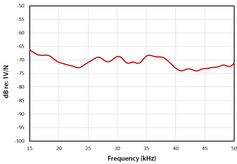
Round-Trip
