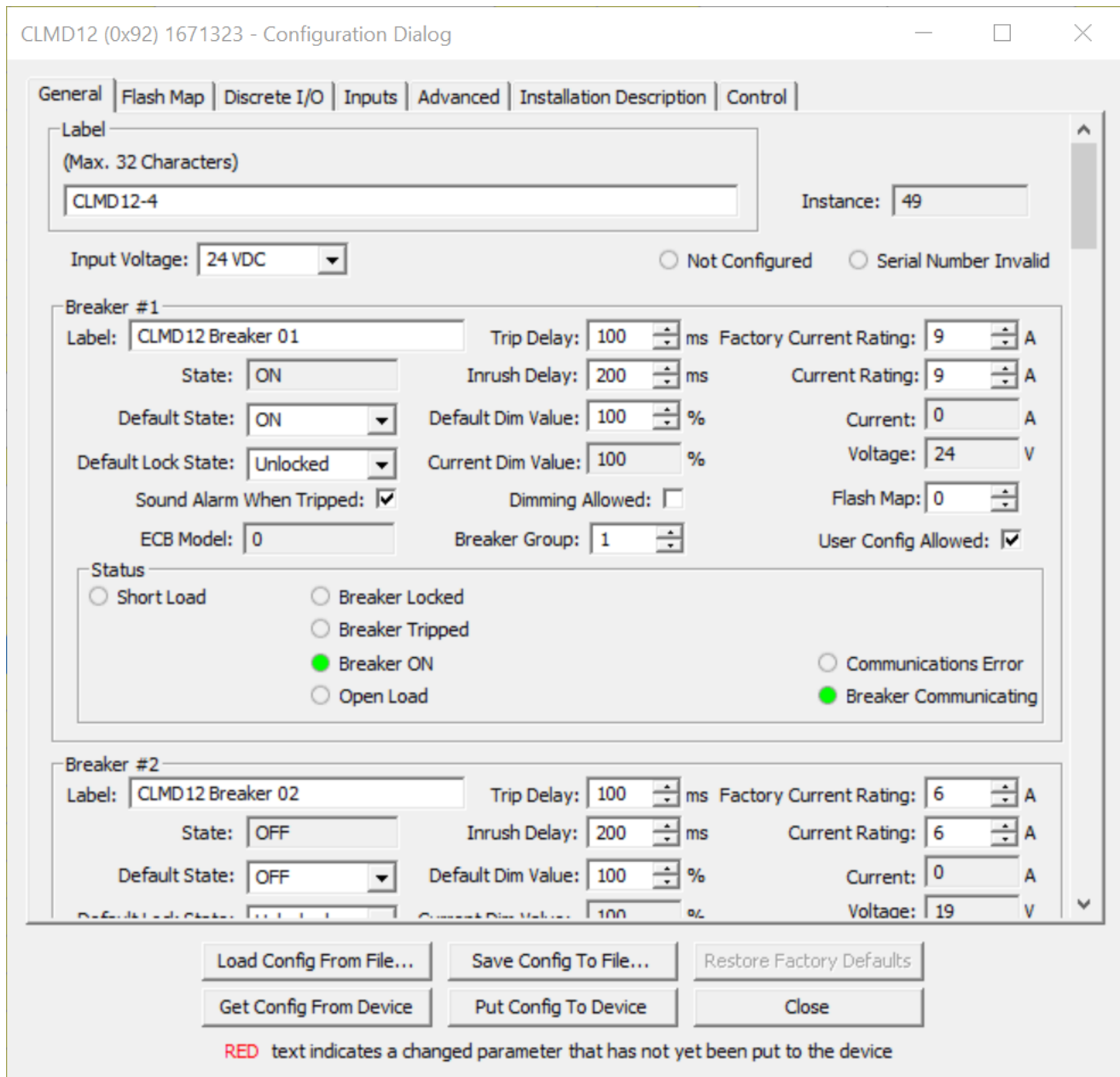
Figure 5 – CLMD12 General Tab
