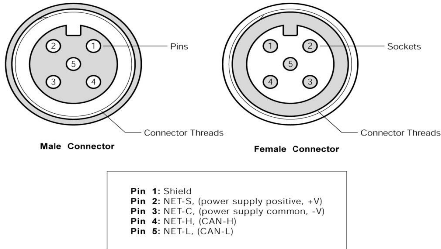
Figure 4 – NMEA 2000® Connector (J3) Face Views
