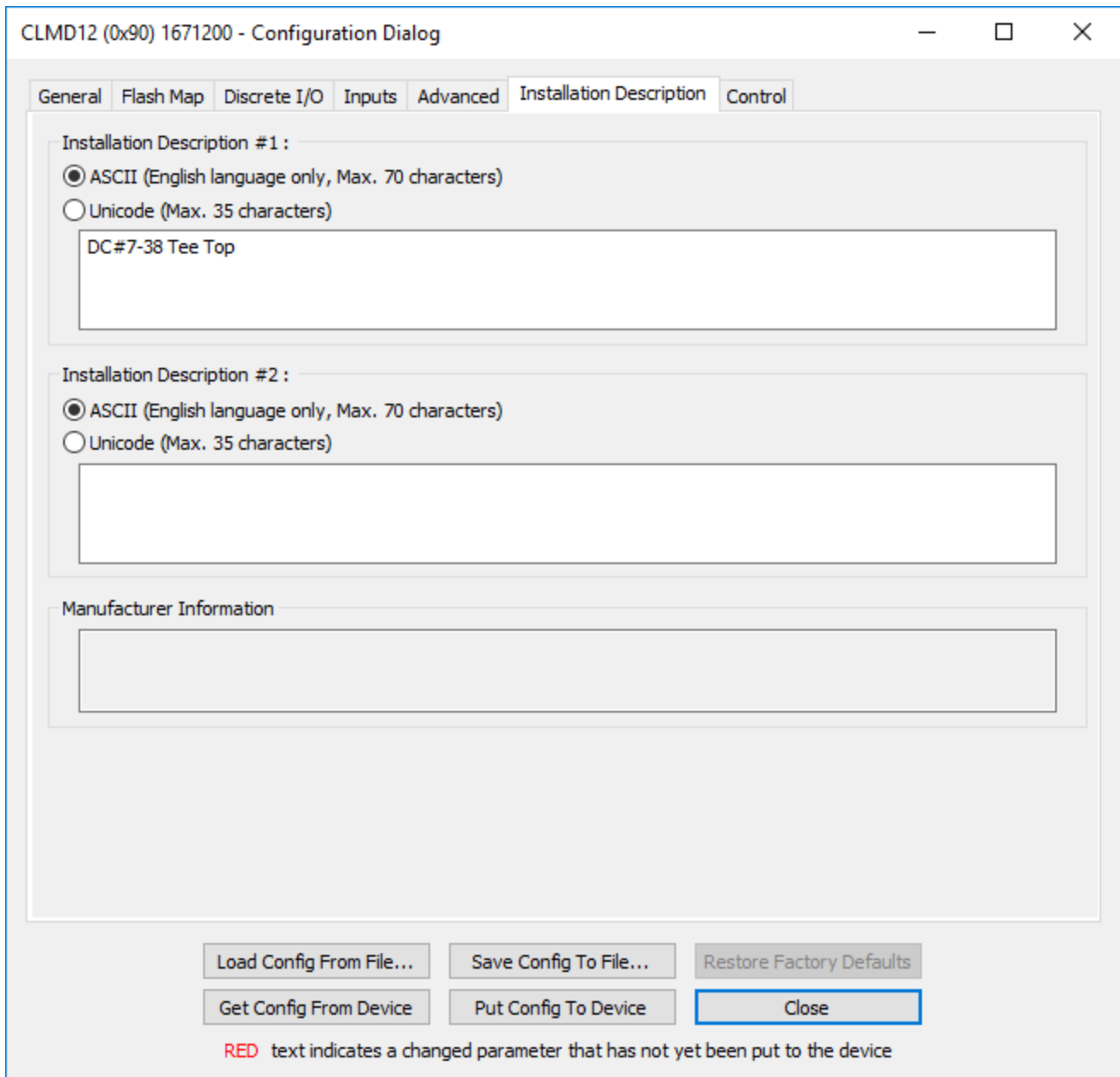
Figure 10 – CLMD12 Installation Description Tab
