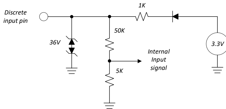
Figure 2 – Discrete Input Impedance Model
