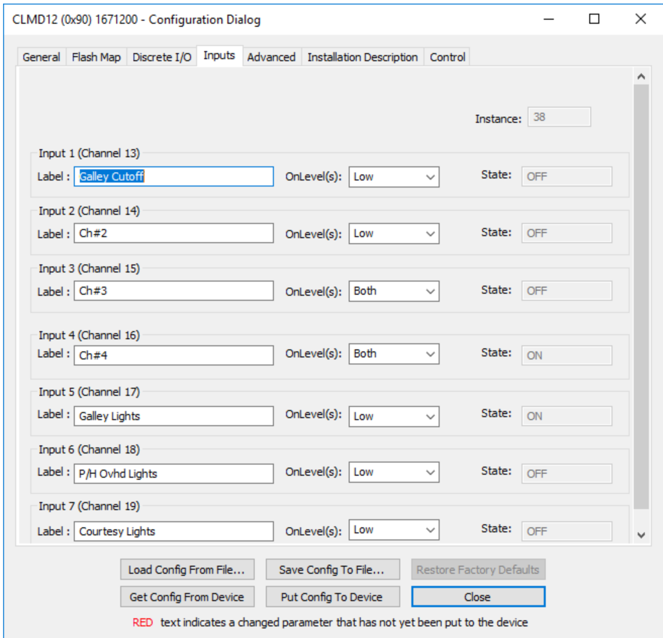
Figure 8 – CLMD12 Inputs Tab
