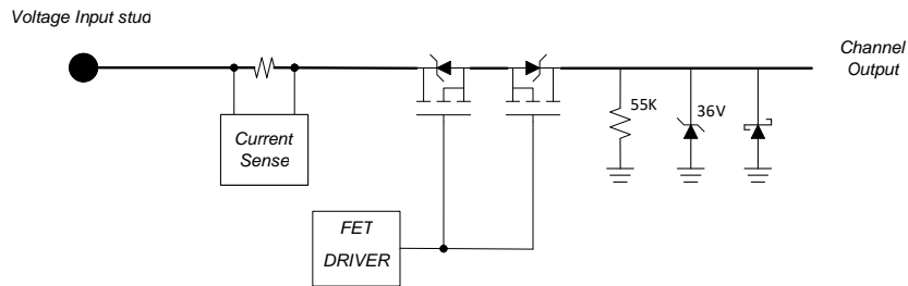
Figure 1 – Output Channel Schematic
