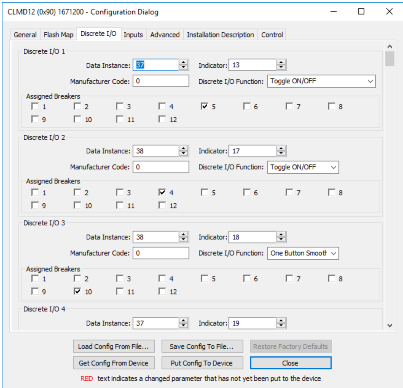
Figure 7 – CLMD12 Discrete I/O Tab
