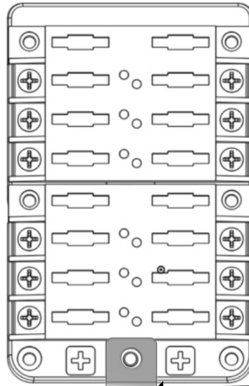
8029B RT Series 12 ATC/ATO Circuit Fuse Block, Ignition Switched (optional Time Delay)
