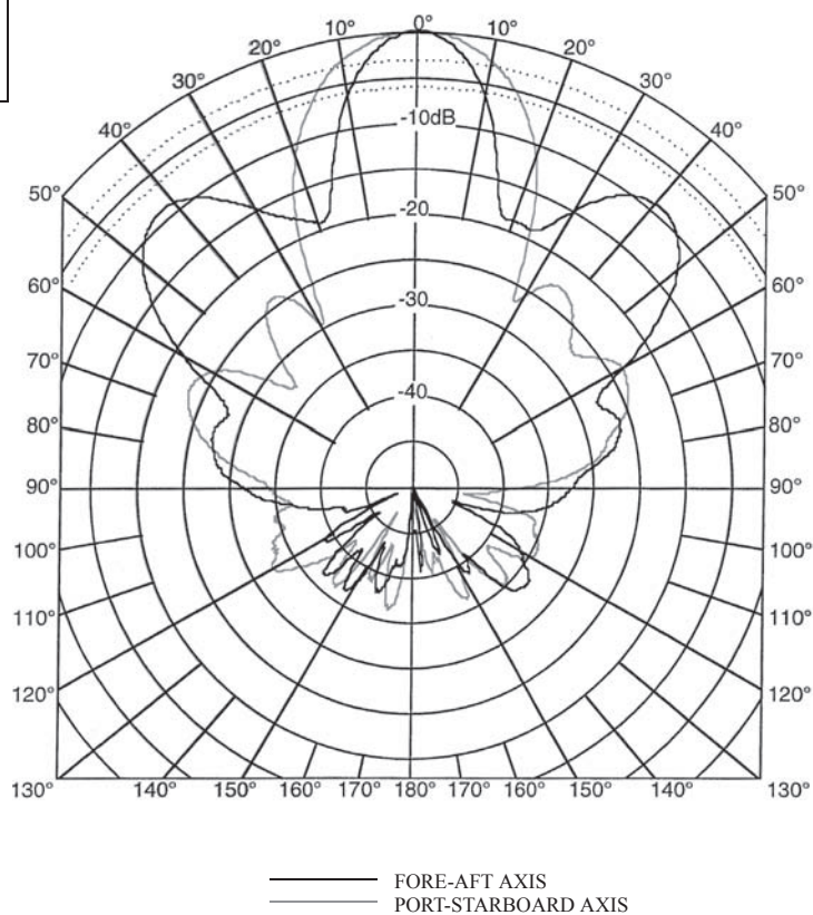
Transmit Radiation Pattern
